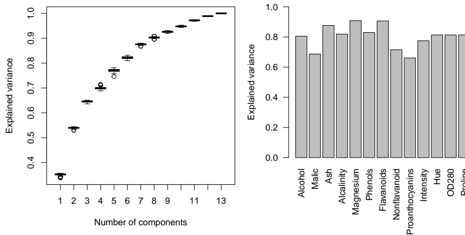
Figure 1: Left: output of pcaCV . Determination of the optimal number of PCs. The data for the boxplots was obtained by 4-fold CV, repeated 50 times. Right: output of pcaVarexp1 . Control the explained variance of each variable.
